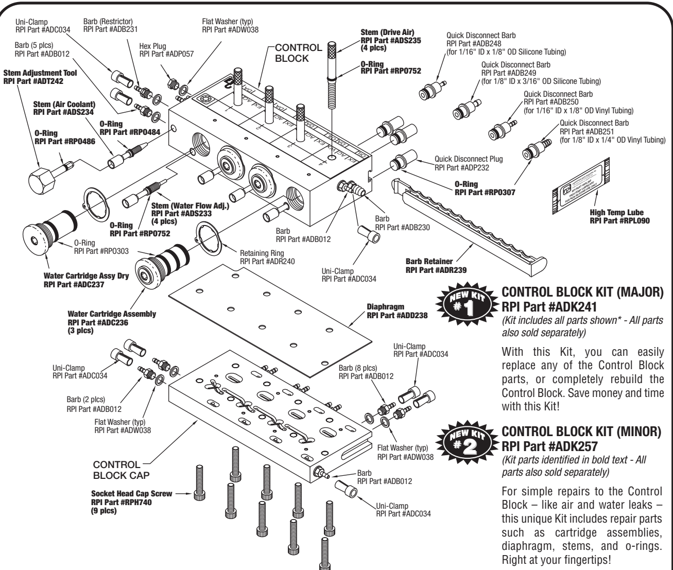
EXPLODED VIEW OF A-dec 500 CONTROL BLOCK ASSEMBLY
