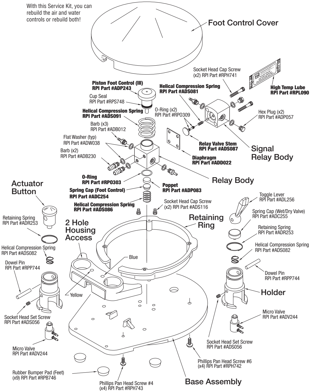
EXPLODED VIEW OF A-dec FOOT CONTROL ASSEMBLY
