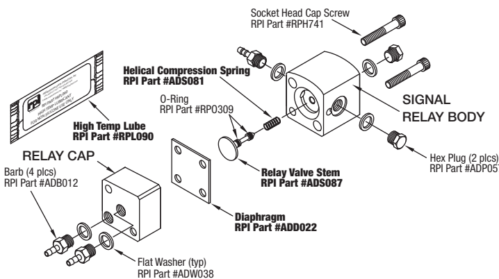
EXPLODED VIEW OF A-dec 500 WATER COOLANT RELAY ASSEMBLY
